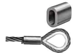
T ferrule (T) (aluminium)
