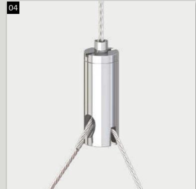
04 Y-Holder type 12 ZW M4ix4 Slit 1.6 mm with set-screw Mx6
