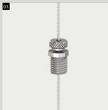
03 Holder type 12 M8x1 A9 with knurled safety-nut M3
